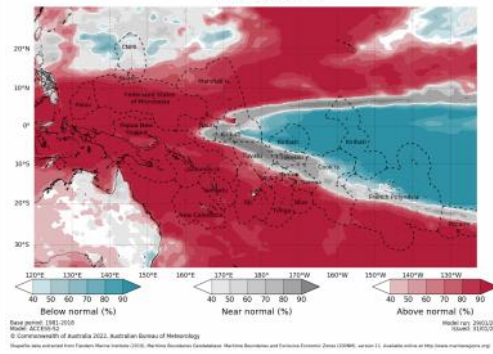
Tercile maximum temperature probabilities for February to April 2022
